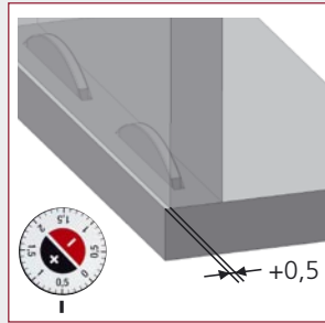
Work piece protruding
